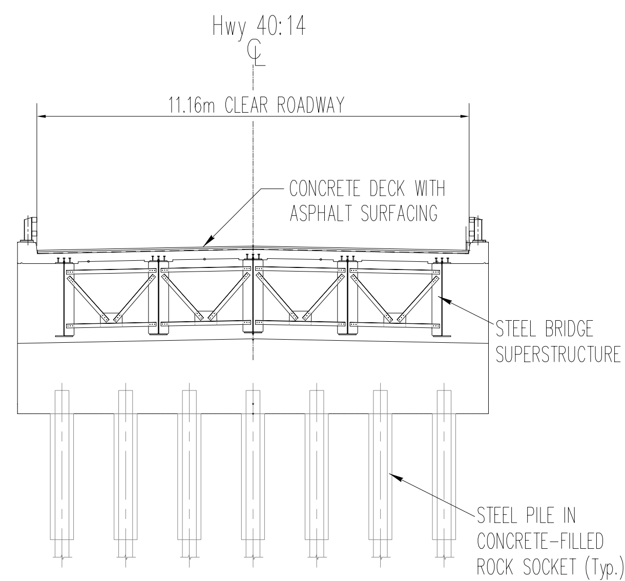
New Roadway Bridge
