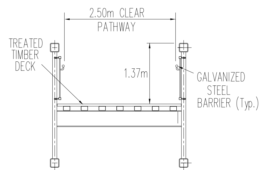
New Pedestrian Bridge
